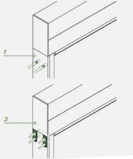
2. fissaggio cassetto a spalletta - guide indipendenti / 2. mounted cassette box in the reveal - the guides do not support it
