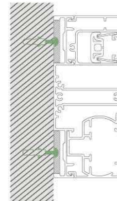
2. fissaggio cassetto a spalletta - guide indipendenti / 2. mounted cassette box in the reveal - the guides do not support it
